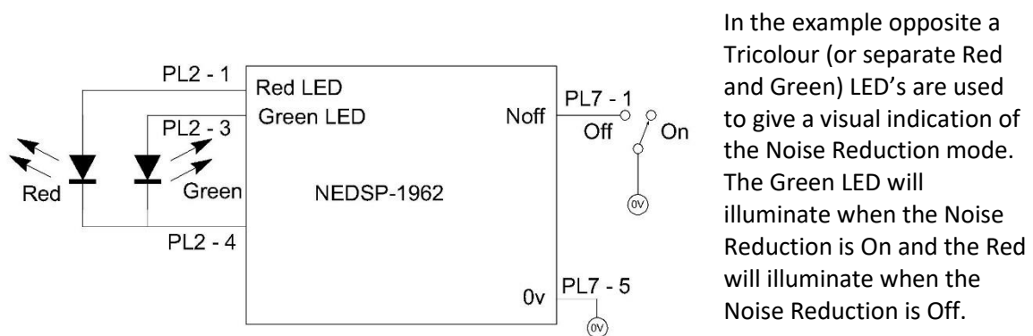
Figure 7. Noise Reduction On/Off with Red/Green LED Status indication
