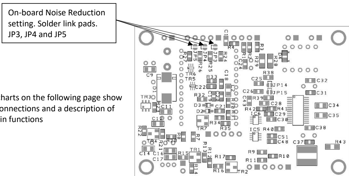
Underside Pictorial
