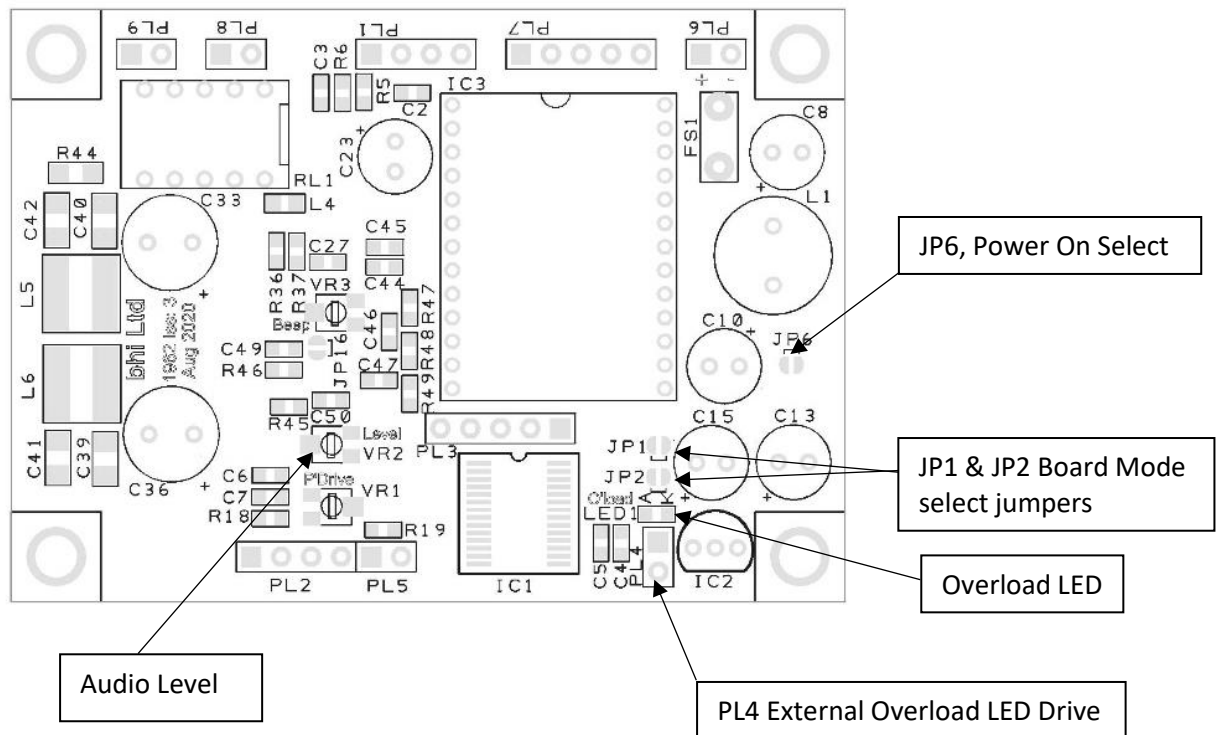
Topside Pictorial
