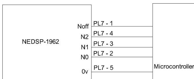
Figure 8. Basic setting using a BCD switch with complementary logic
