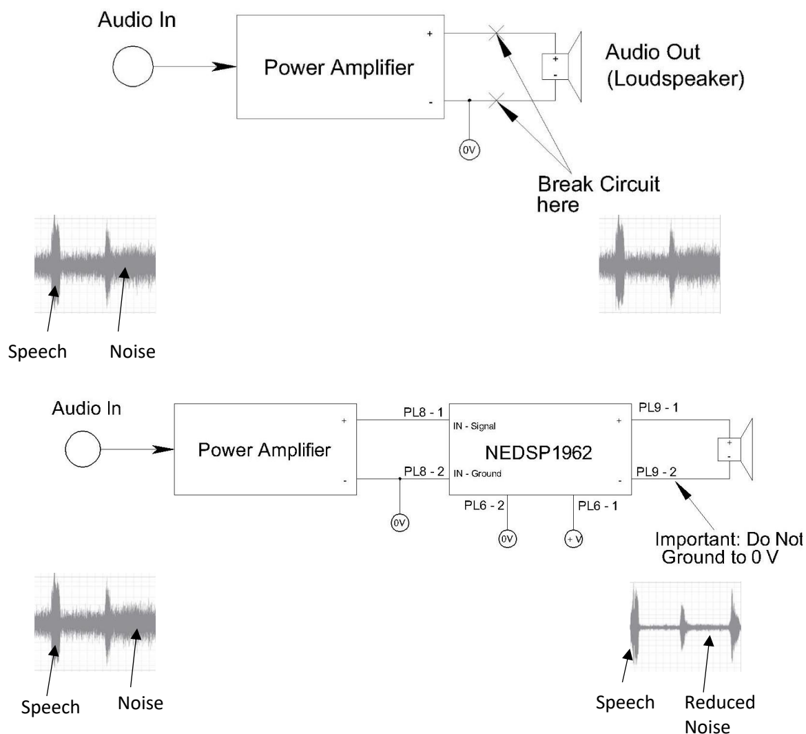
Figure 6. Basic connection diagram
