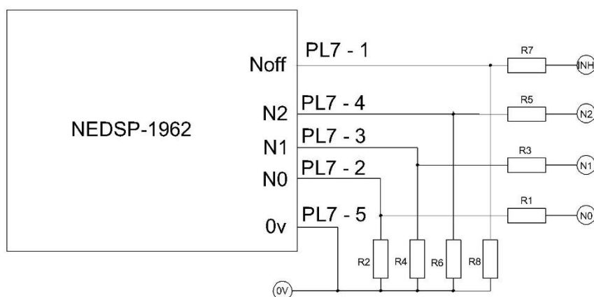
Figure 10 – Using a Resistor Divider circuit to allow operation with higher voltage logic
