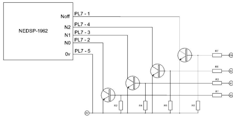
Figure 11. Control of settings using a Transistors
